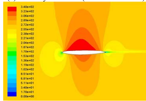
Figure 14: Results for optimized NACA 0012 Airfoil, M = 0.85 , \alpha = 1.5 degree
