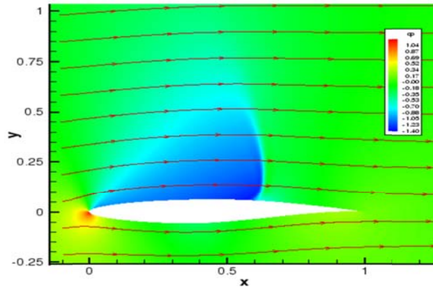
Figure 1: RAE 2822 airfoil: Pressure contours and streamlines at M = 0.75 , Re = 6.2 \times 10^6 , \alpha = 2.8^\circ [11]
