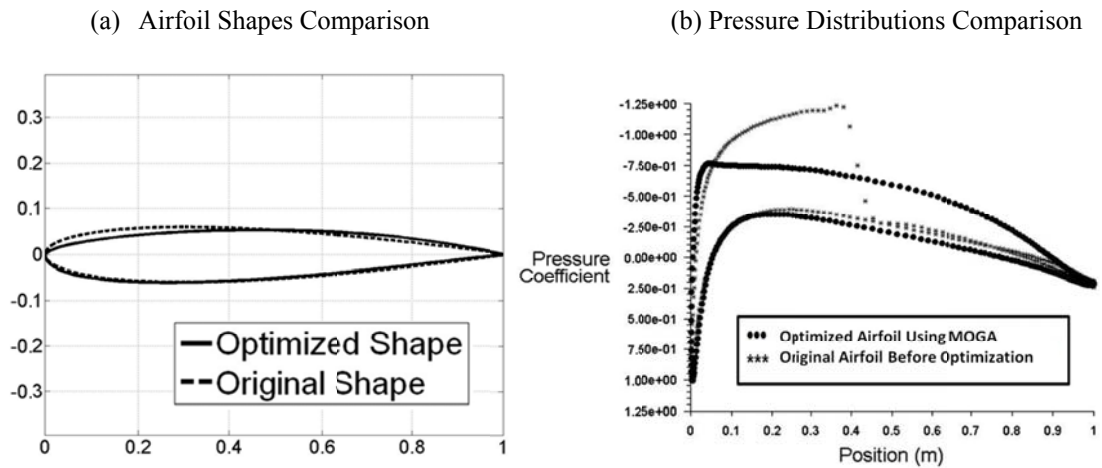
Figure 17: Comparison of original and optimized NACA 0012 airfoil shapes and pressure distribution; M = 0.75 , \alpha = 2 degree
