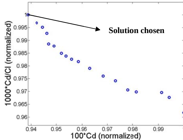
Figure 7: Pareto solutions for RAE 2822 airfoil
