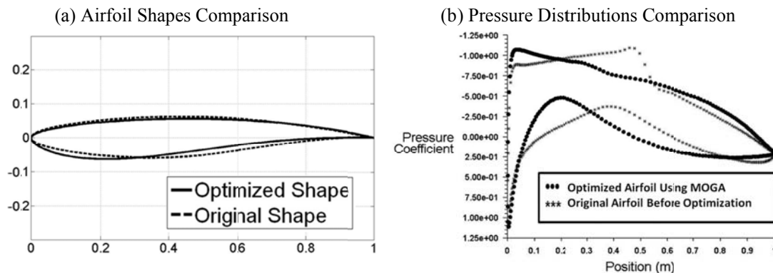
Figure 15: Comparison of original and optimized RAE 2822 airfoil shapes and pressure distributions; M = 0.73 , \alpha = 2 degree
