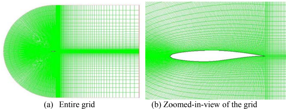
Figure 8: C-Grid around the RAE 2822 airfoil
