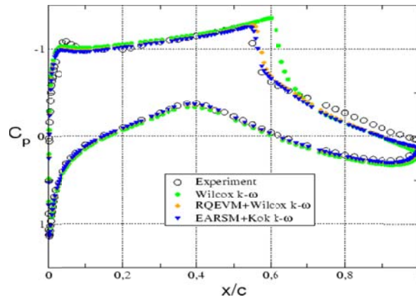
Figure 2: RAE 2822 airfoil: Pressure distribution at M = 0.75 , Re = 6.2 \times 10^6 , \alpha = 2.8^\circ [11]
