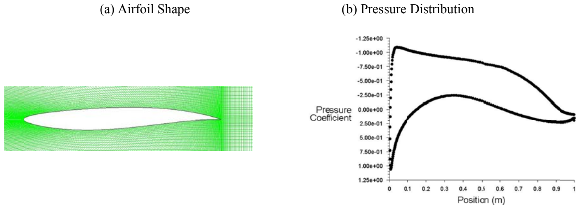
Figure 11: Results for optimized RAE 2822 airfoil, M = 0.73 , \alpha = 2 degree
