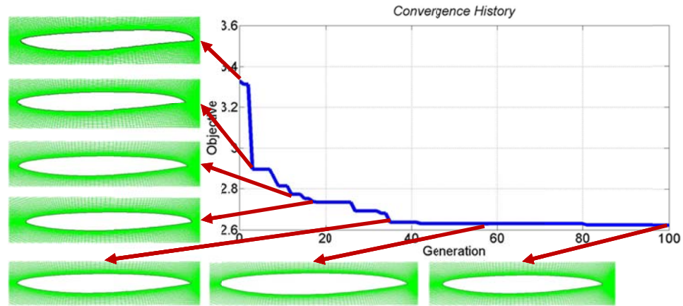
Figure 10: Convergence history of NACA 0012 II optimized airfoil using the GA algorithm
