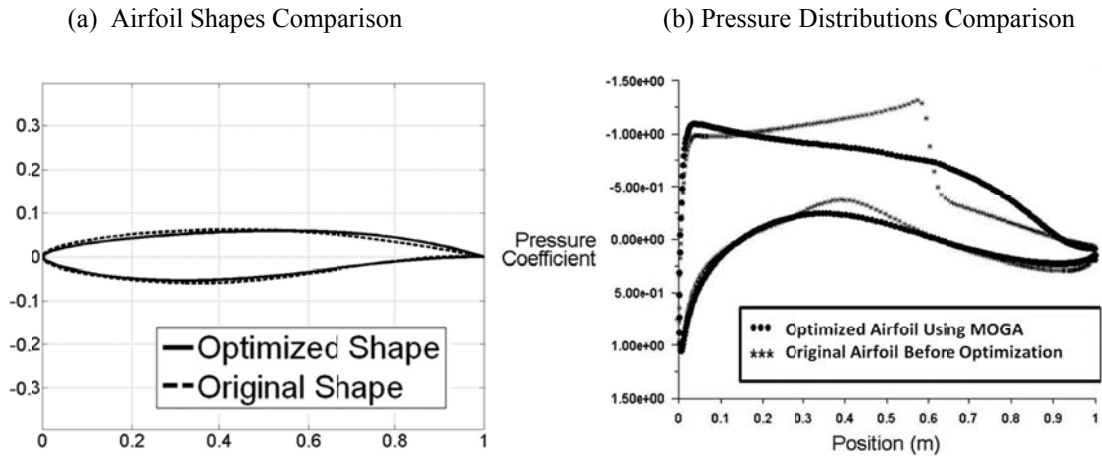
Figure 16: Comparison of original and optimized RAE 2822 airfoil shapes and pressure distributions; M = 0.75 , \alpha = 2.8 degree
