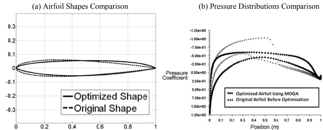
Figure 18: Comparison of original and optimized NACA 0012 airfoil shapes and pressure distributions; M = 0.8 , \alpha = 1.5 degree
