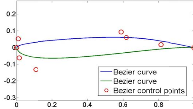
Figure 5: Example of Bezier curves and Bezier control points
