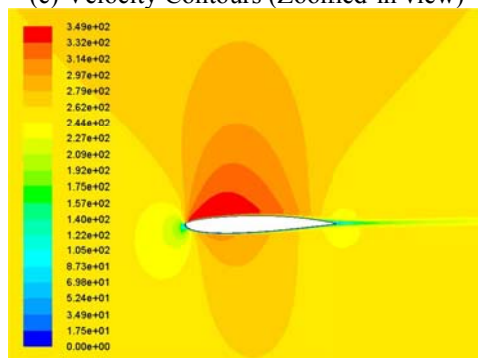
Figure 13: Results for optimized NACA 0012 Airfoil, M = 0.75 , \alpha = 2 degree
