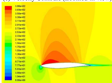
Figure 12: Results for optimized RAE 2822 Airfoil, M = 0.75 , \alpha = 2.8 degree
