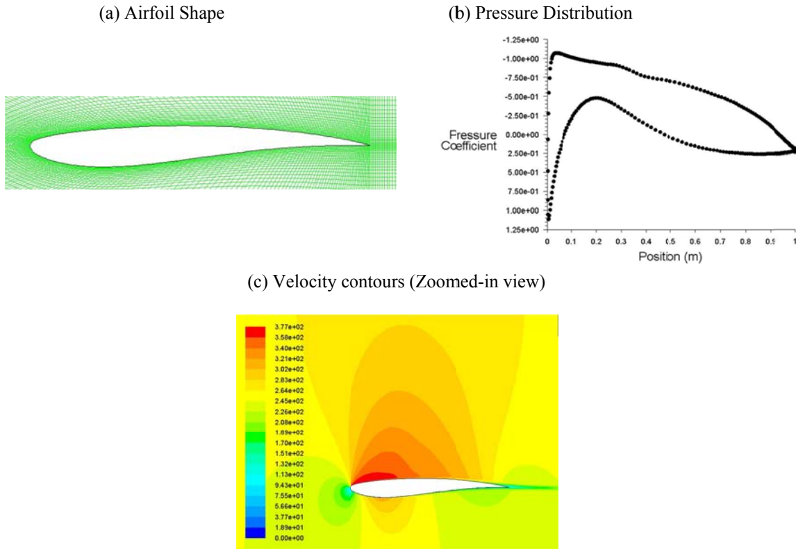
Figure 11: Results for optimized RAE 2822 airfoil, M = 0.73 , \alpha = 2 degree
