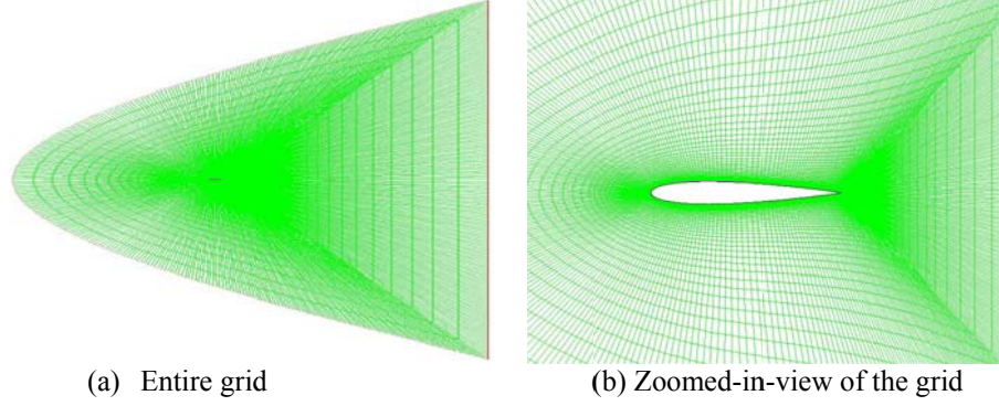
Figure 9: C-Grid around the NACA 0012 airfoil
